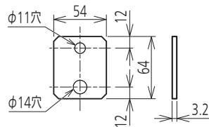
2穴平座金 (同梱部品)
